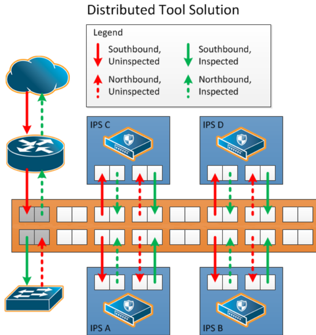
Figure 284: Multiple Tool Arrangement
