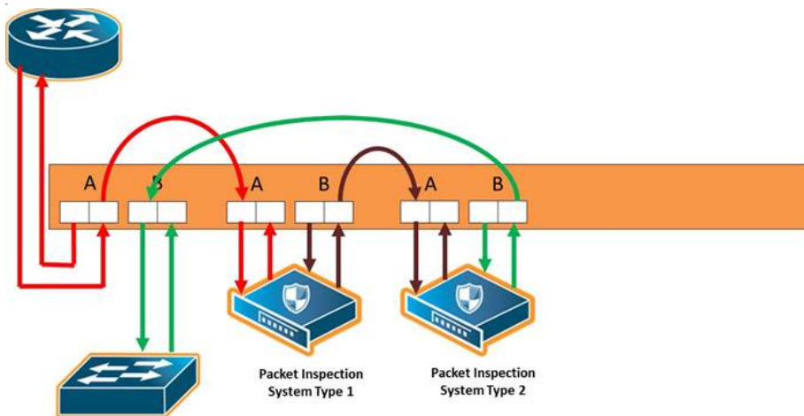
Figure 304: Inline Serial Tools
