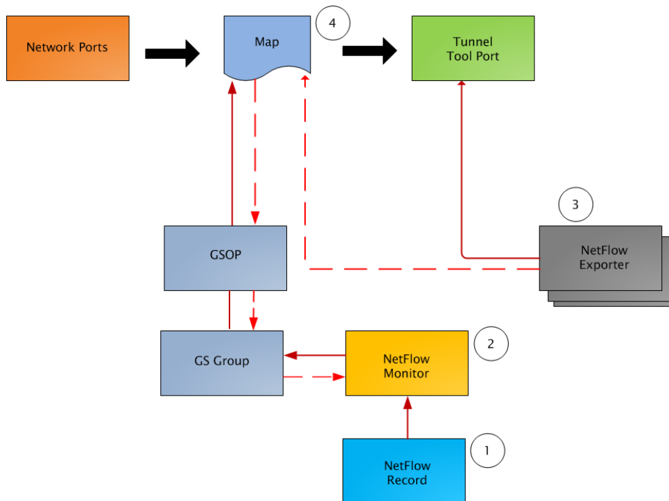
Figure 431: NetFlow Generation Components
