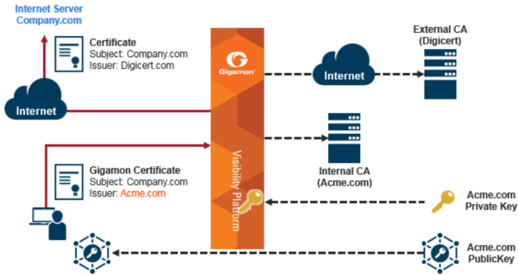
Figure 443: Outbound Deployment of Inline SSL Decryption
