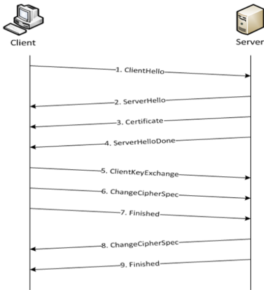
Figure 472: Basic SSL Handshake
