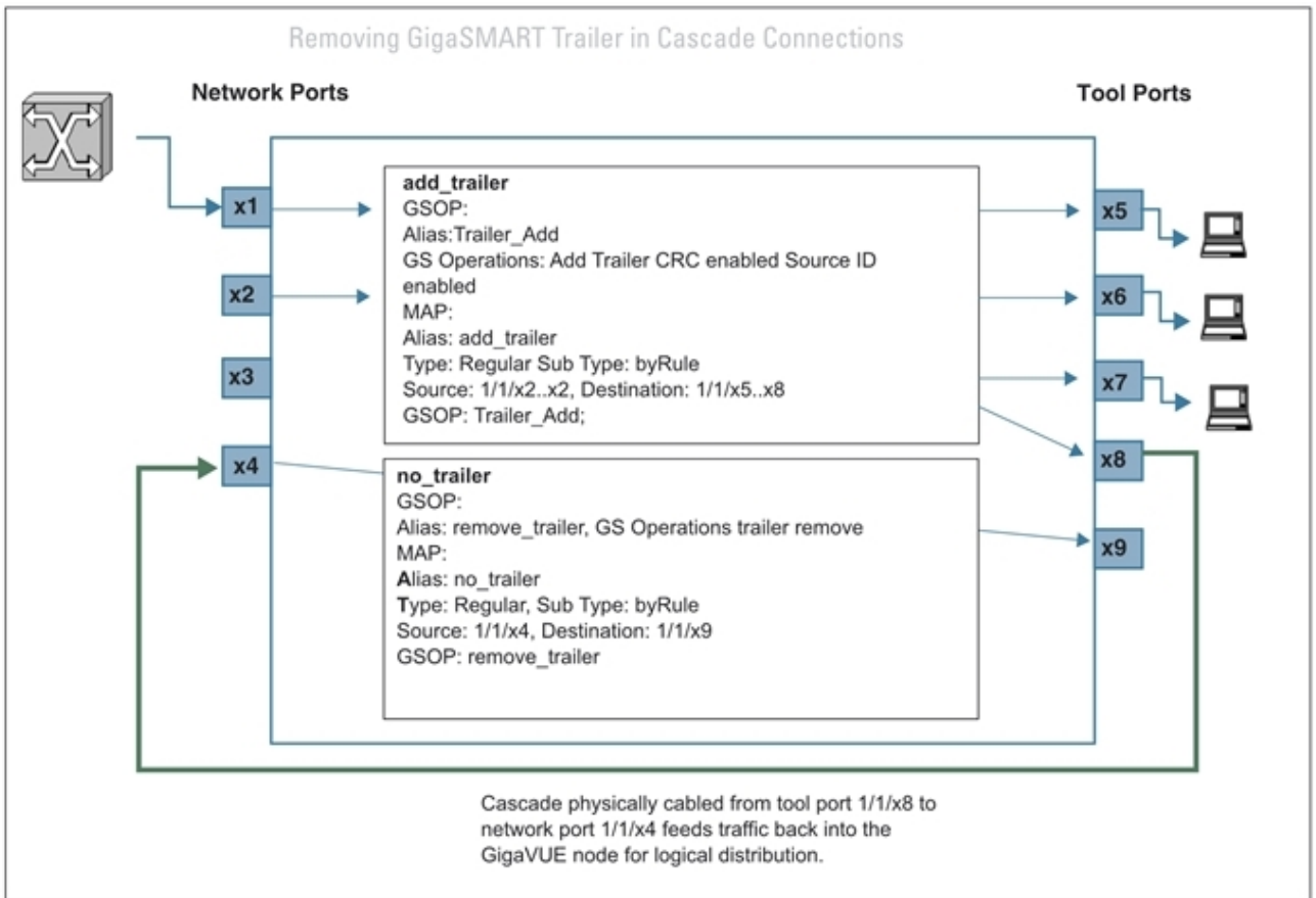
Figure 522: Removing the GigaSMART Trailer from a Cascade Connection
