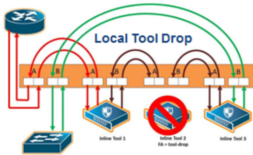
Figure 310: Inline Tool Series Local Tool Drop Failover Action
