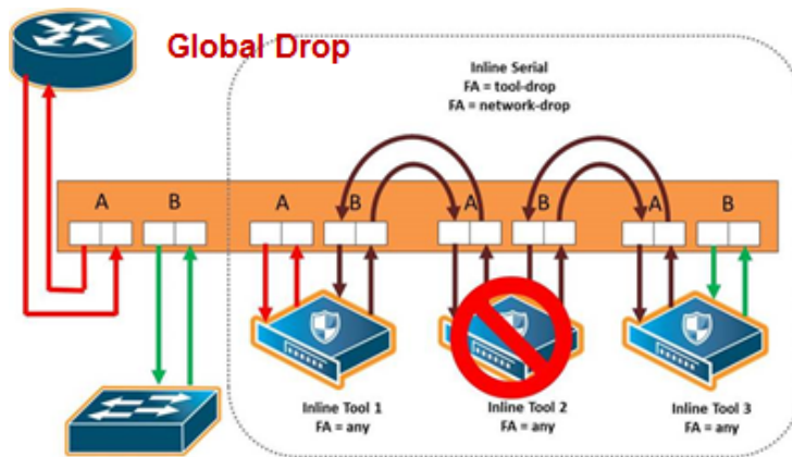
Figure 308: Inline Tool Series Global Drop Failover Action
