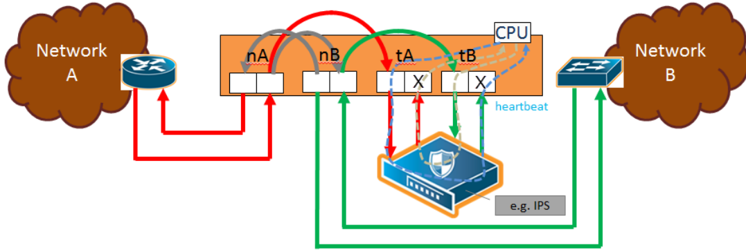
Figure 292: Traffic Path of Monitoring
