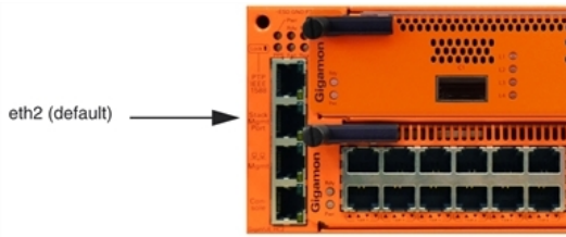
Figure 454: Stack Port Location on GigaVUE-HC2 Front
