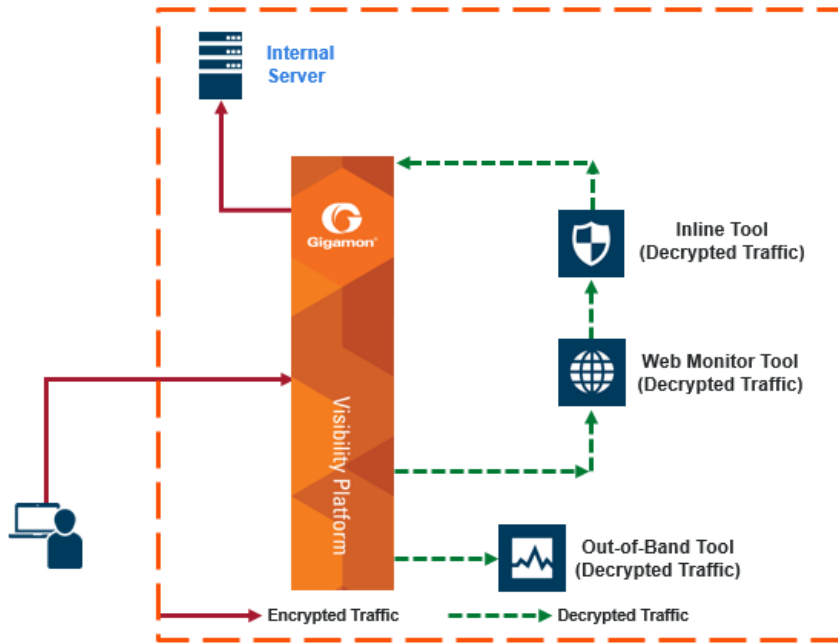
Figure 442: Inbound Deployment of Inline SSL Decryption
