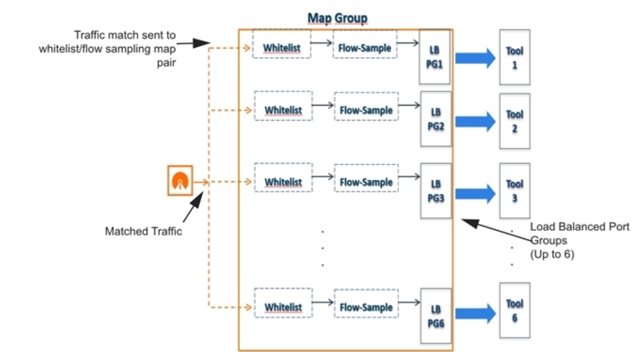
Figure 386: GTP Overlap Flow Sampling Map Groups
