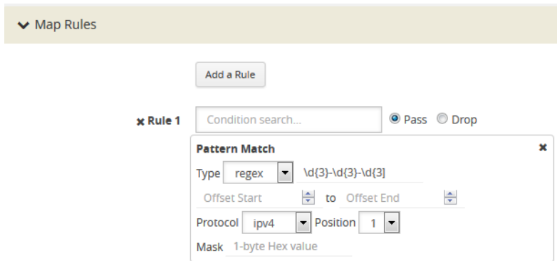
Figure 394: Pattern Match with Type RegEx
