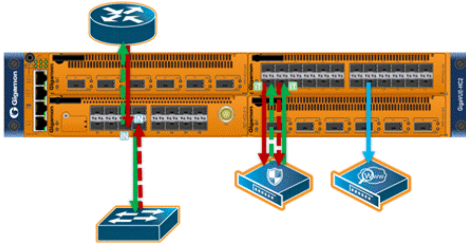
Figure 326: Logical Bypass Without Bypass Combo Module
