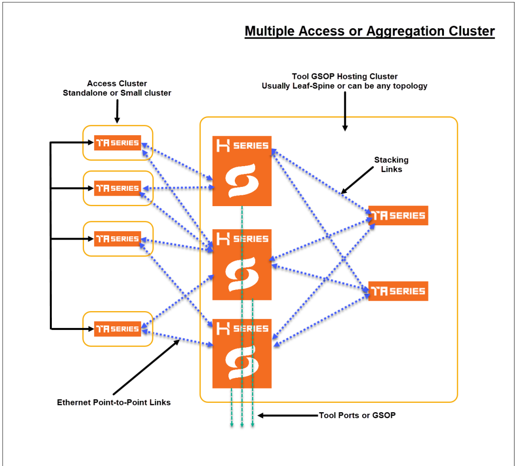
Figure 337: Multiple Access Clusters
