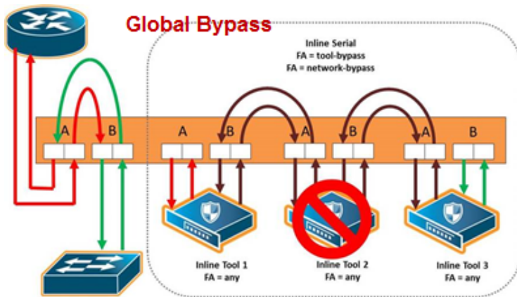
Figure 306: Inline Tool Series Global Bypass Failover Action
