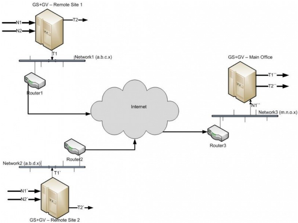
Figure 495: L2GRE Tunnel Encapsulation/Decapsulation
