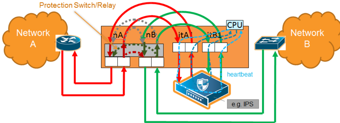
Figure 280: Physical Bypass Protection
