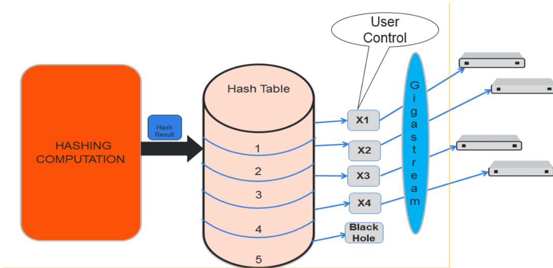
Figure 212: Controlled GigaStream Example
