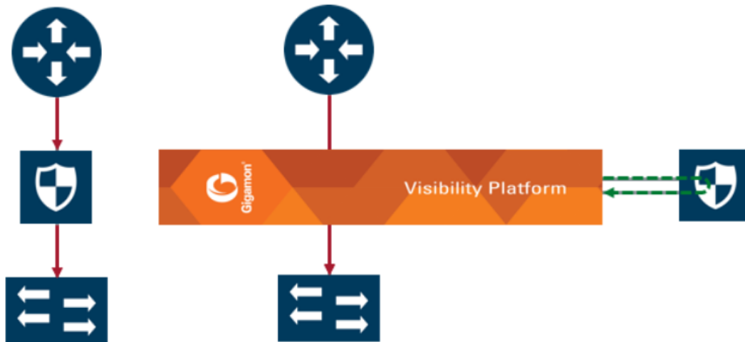
Figure 451: Simple Inline Tool Arrangement
