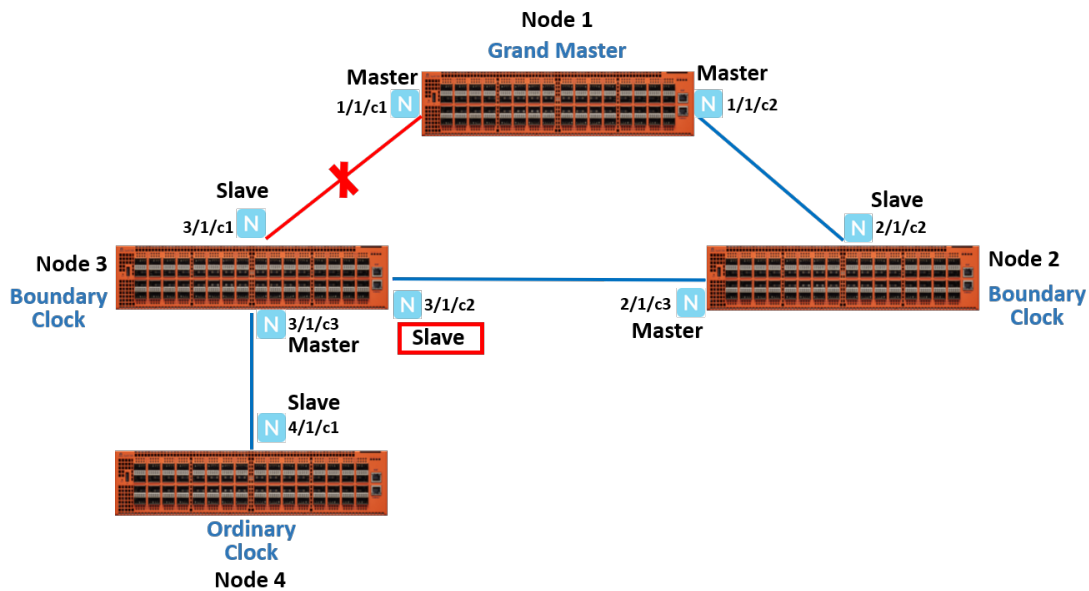
Figure 331: PTP State Transition
