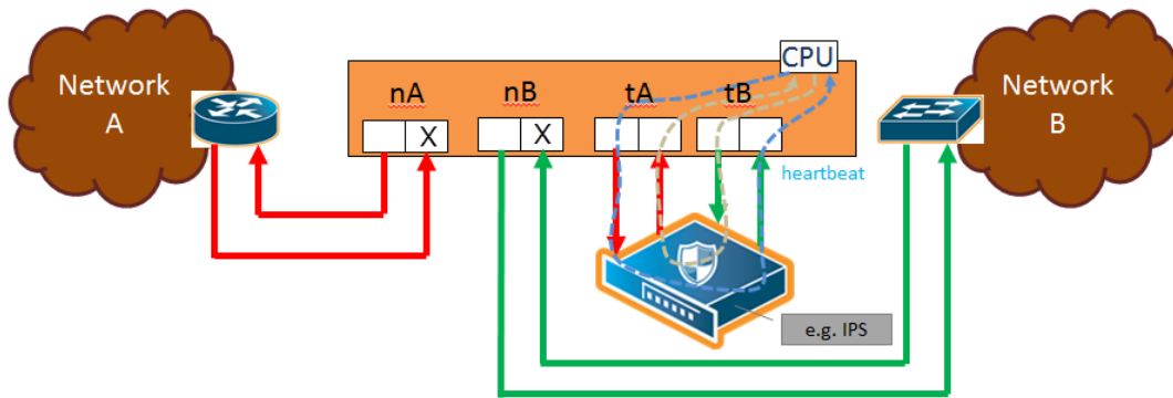
Figure 290: Traffic Path of Drop
