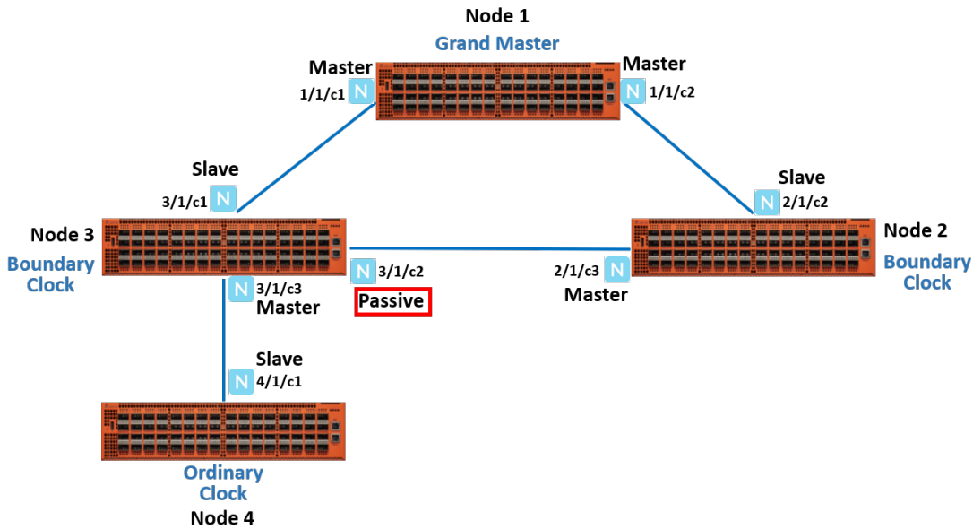
Figure 330: PTP Deployment
