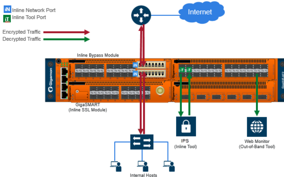
Figure 444: GigaVUE Modules: GigaSMART and Inline Bypass
