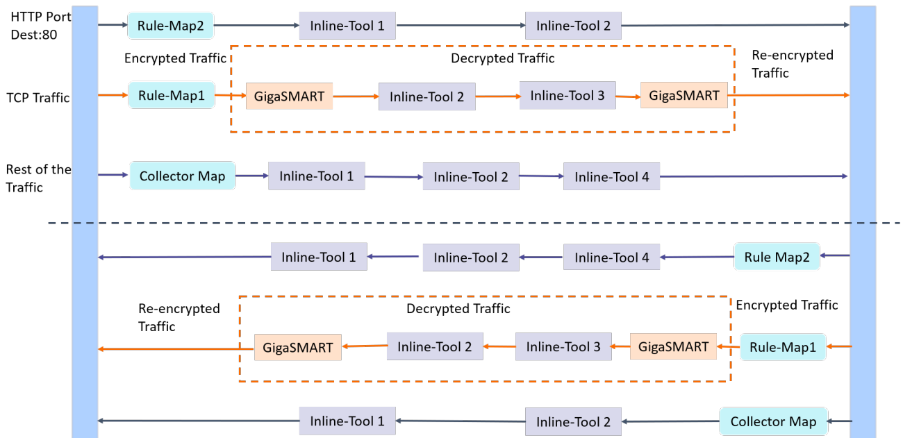
Figure 274: Flexible Inline Decryption Solution
