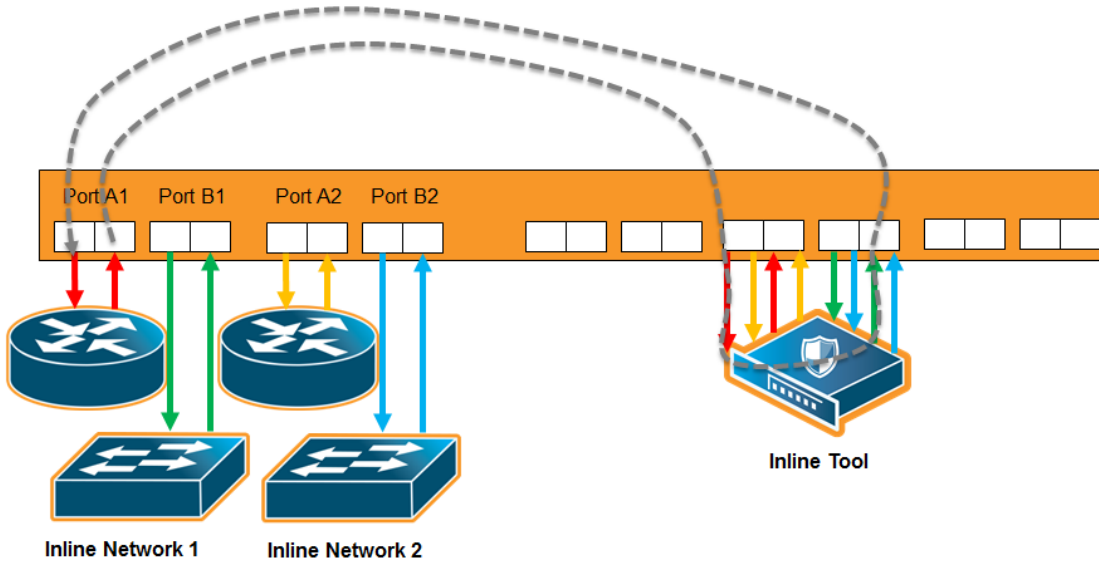
Figure 286: Inline Network Group
