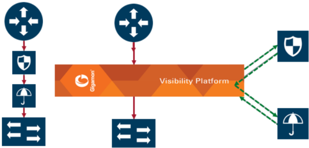
Figure 453: Serial Inline Tool Arrangement
