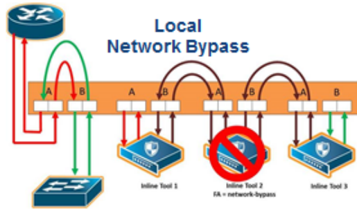
Figure 311: Inline Tool Series Local Network Bypass Failover Action
