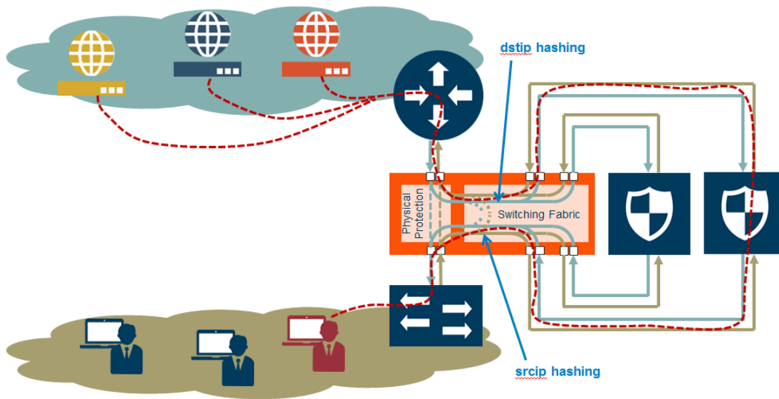
Figure 303: Asymmetrical Hashing
