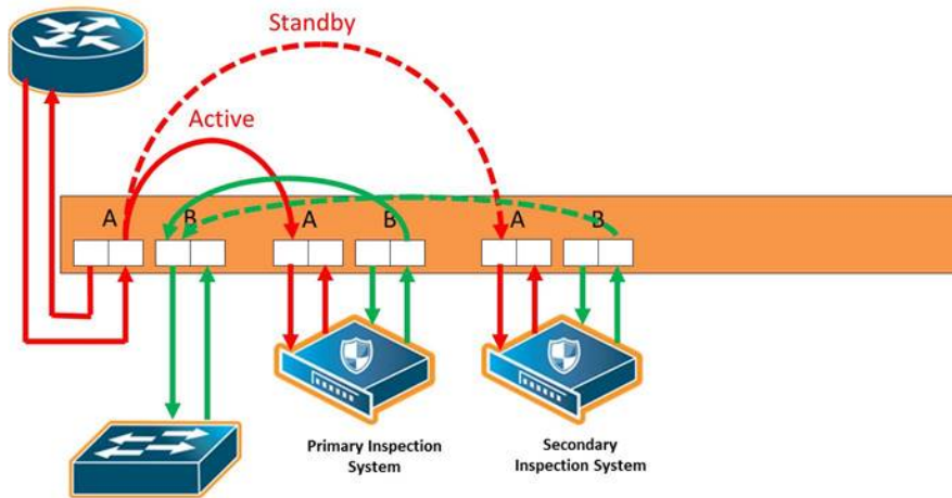
Figure 301: Inline Tool Group With Spare, Redundant 1+1 Scenario
