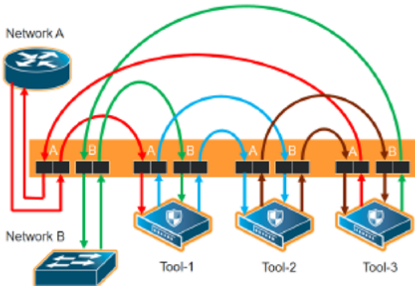
Figure 317: Inline Tool Series Per-Direction: Forward
