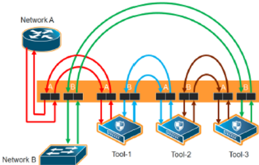
Figure 316: Inline Tool Series Per-Direction: Reversed
