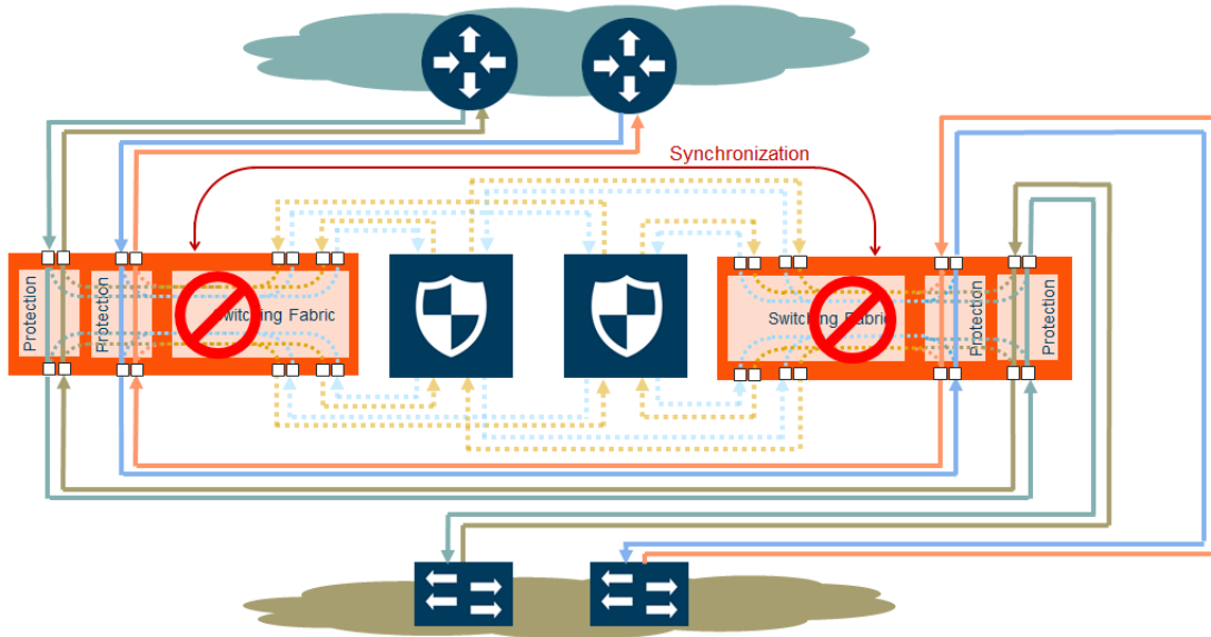
Figure 324: Both Nodes Fail; No Traffic Monitoring
