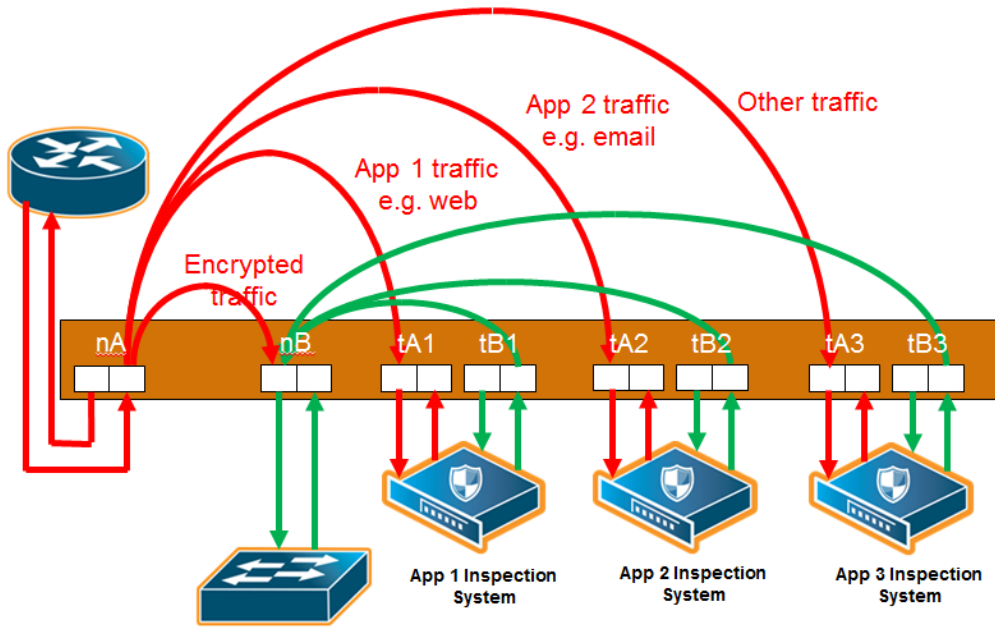
Figure 287: Inline Flow Mapping® Based Traffic Distribution
