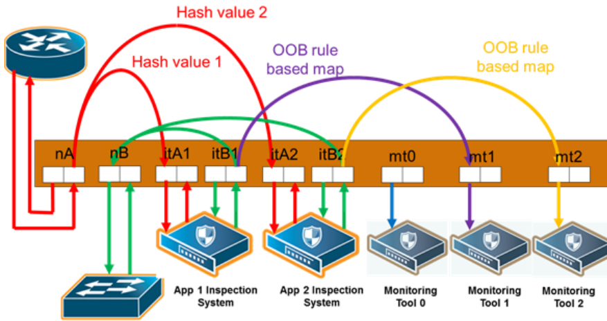
Figure 319: Out-of-Band Rule-Based Maps
