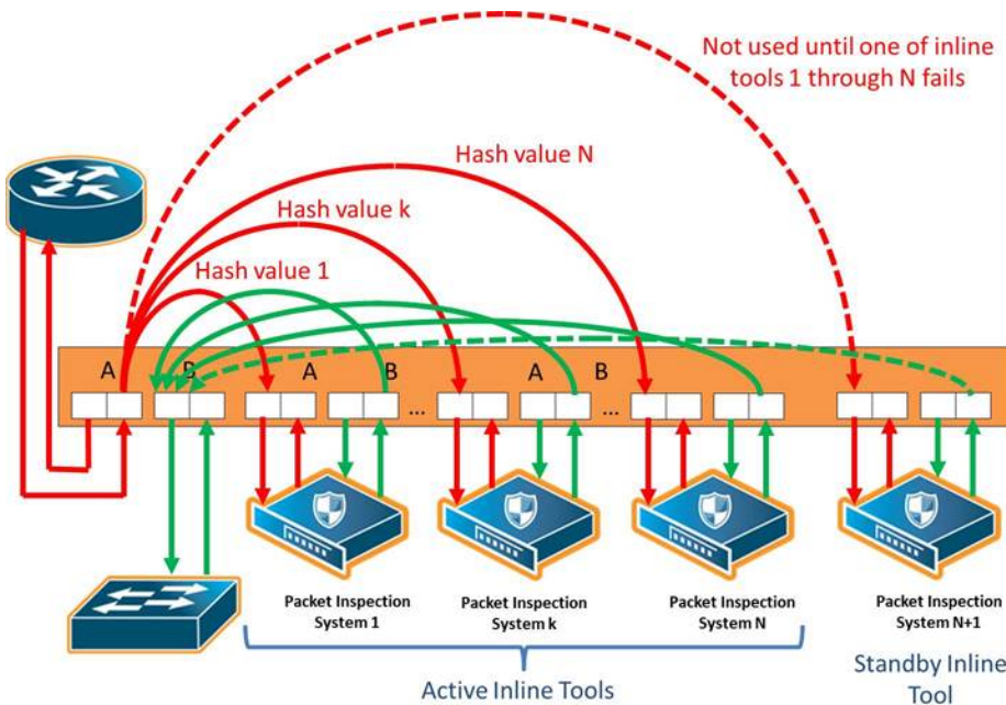
Figure 302: Inline Tool Group With Spare, Redundant N+1 Scenario
