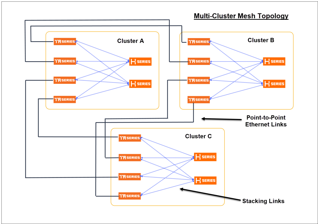
Figure 338: Multi-Cluster Mesh
