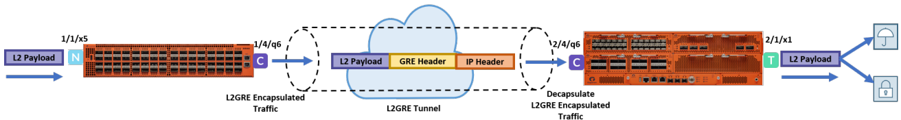
Figure 224: L2GRE Tunnel Encapsulation and Decapsulation
