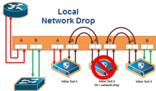
Figure 312: Inline Tool Series Local Network Drop Failover Action
