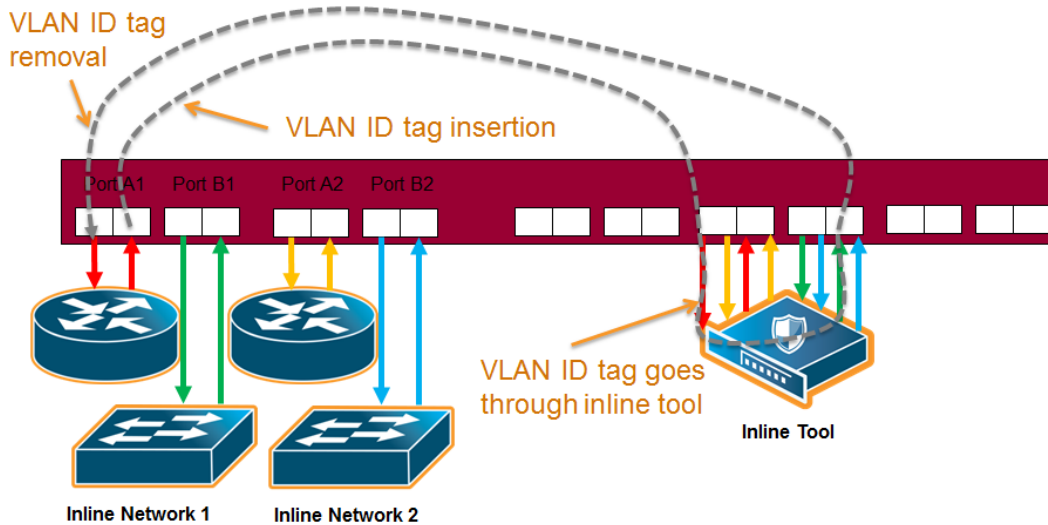
Figure 294: Inline Network Group Many-to-One
