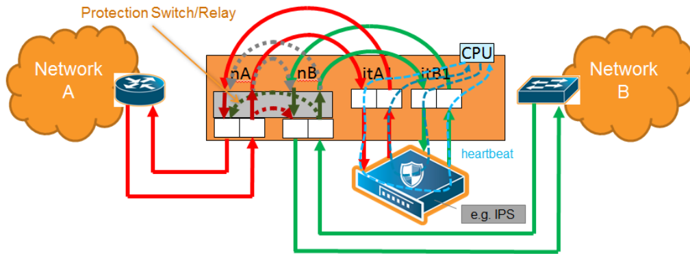
Figure 283: Simple Configuration
