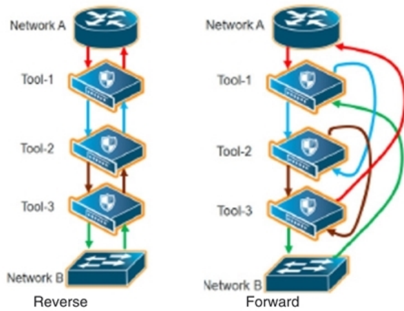
Figure 315: Inline Tool Series Per-Direction Order: Simplified Reverse and Forward
