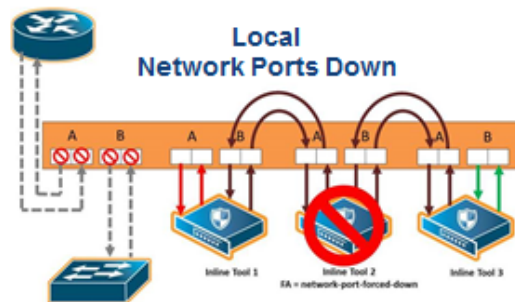
Figure 313: Inline Tool Series Local Network Ports Forced Down Failover Action
