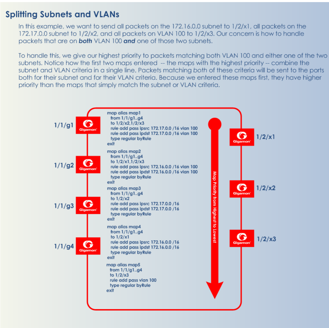
Figure 238: Sending Subnets and VLANs to Different Ports
