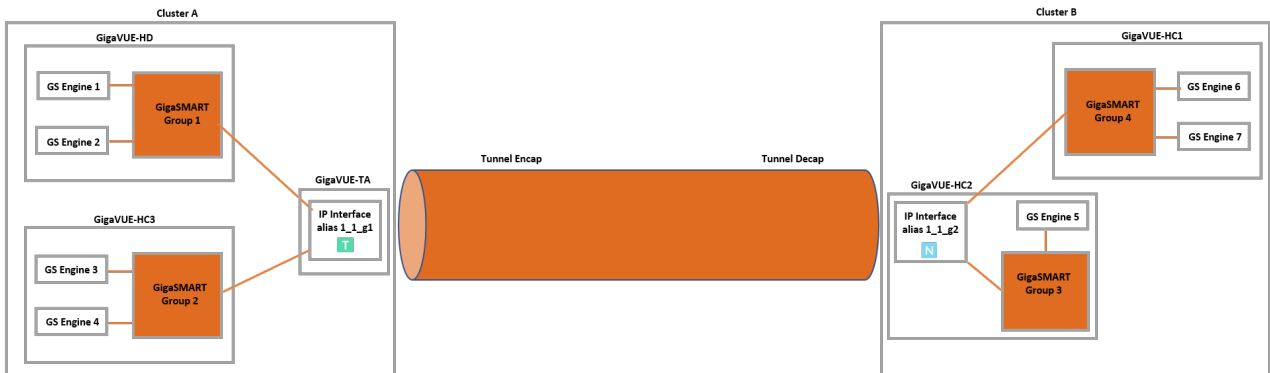
Figure 202: Tunnel Centralization
