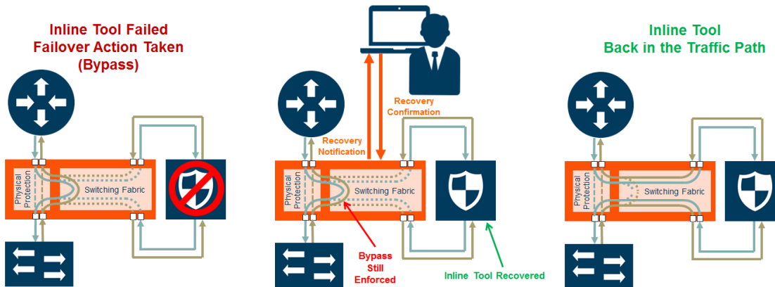
Figure 297: Automatic and Manual Inline Tool Recovery from Failover
