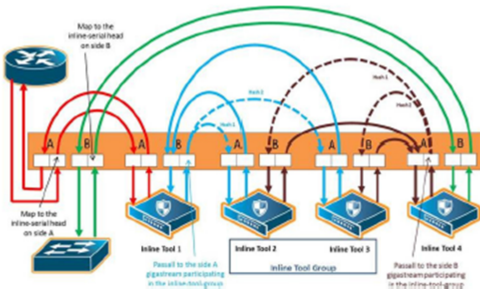
Figure 305: Inline Tool Series, Including Inline Tool Group
