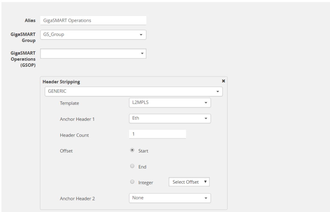
Figure 419: Generic Header Stripping - L2 MPLS
