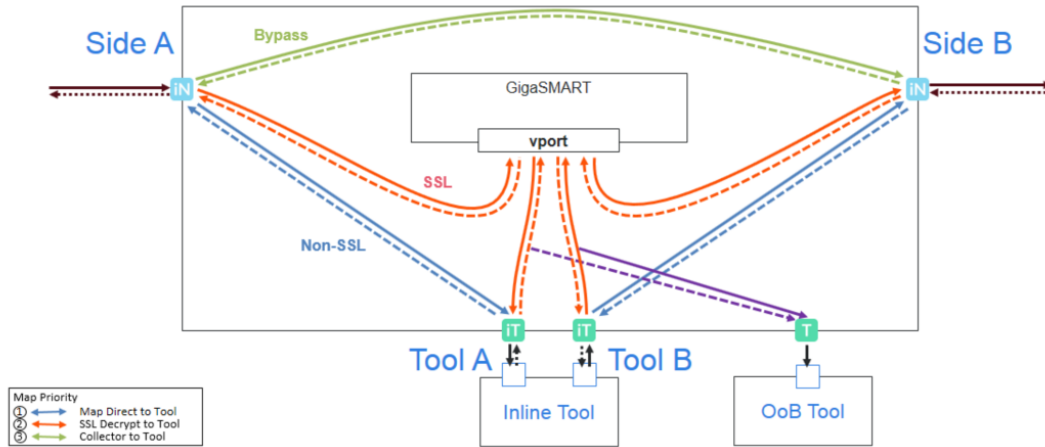
Figure 445: Packet Flow for Inline SSL Decryption
