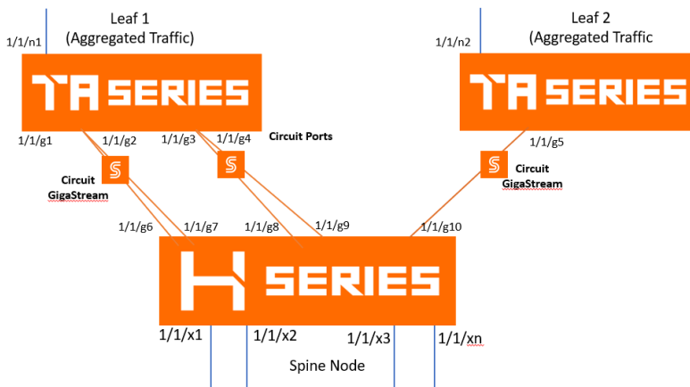
Figure 340: Circuit GigaStreams in Fabric Maps
