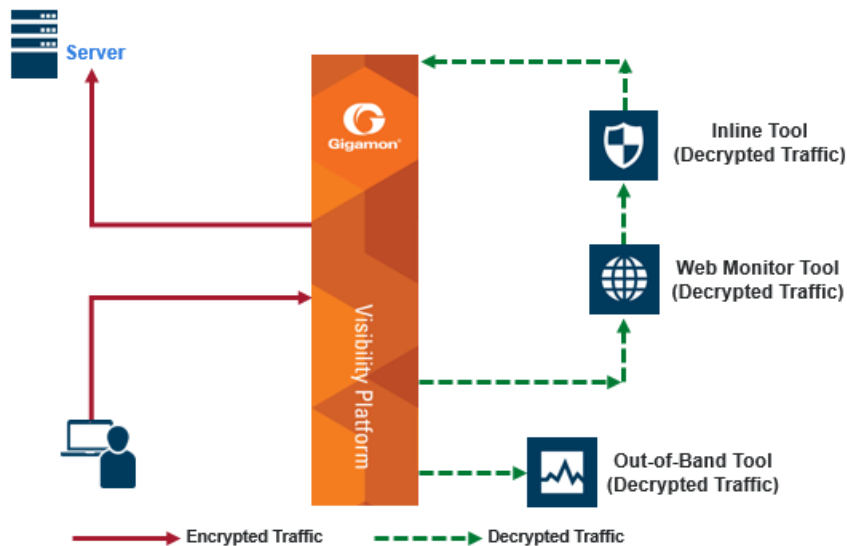
Figure 441: Inline SSL Decryption Example, Outbound
