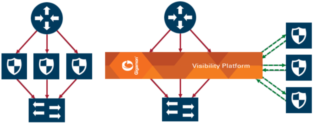
Figure 452: Multiple Inline Tool Arrangement
