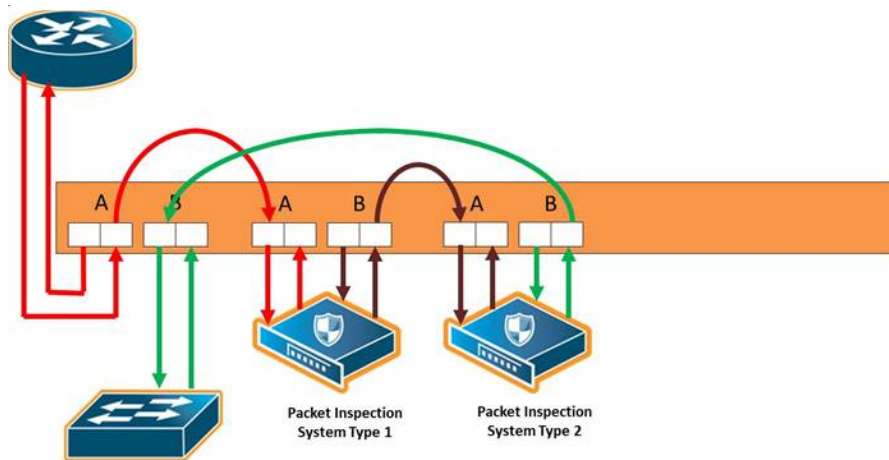
Figure 285: Inline Tool Series
