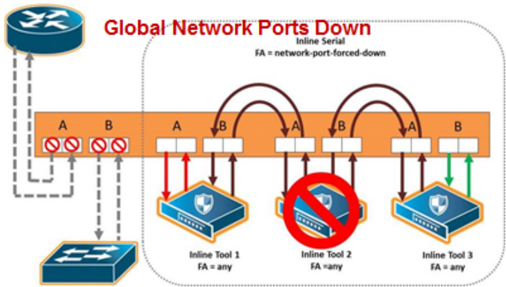
Figure 307: Inline Tool Series Global Network Ports Forced Down Failover Action
