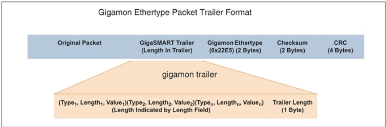
Figure 523: GigaSMART Trailer Format
