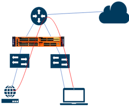
Figure 450: Inline SSL Inline Network Group Configuration
