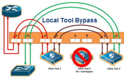
Figure 309: Inline Tool Series Local Tool Bypass Failover Action
