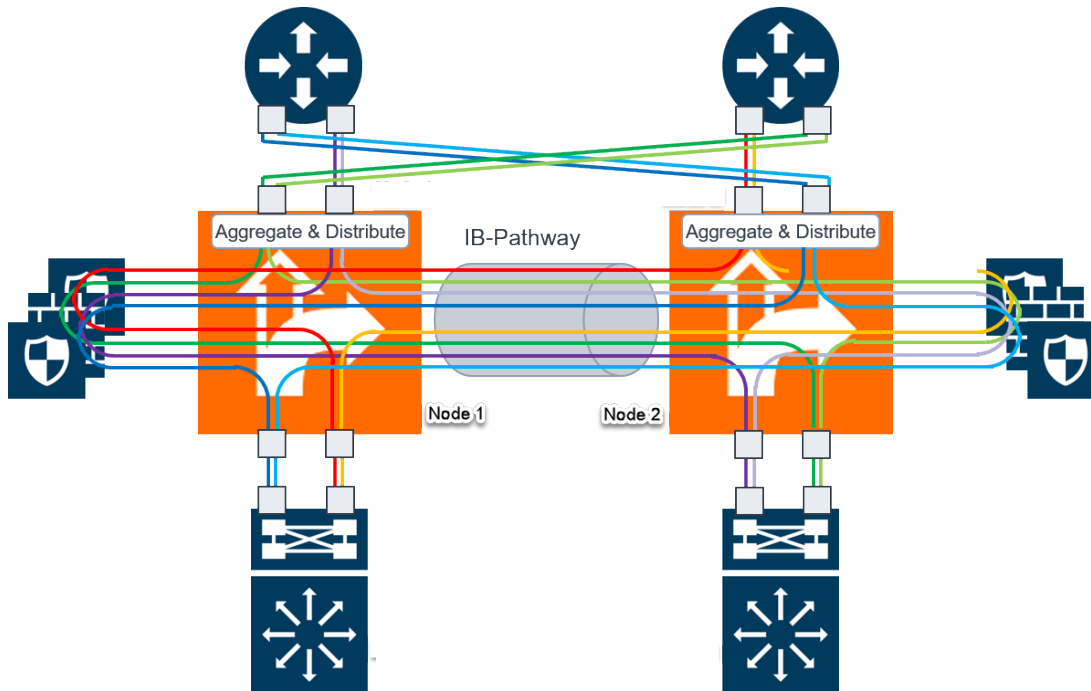
Figure 272: Resilient Inline Architecture
