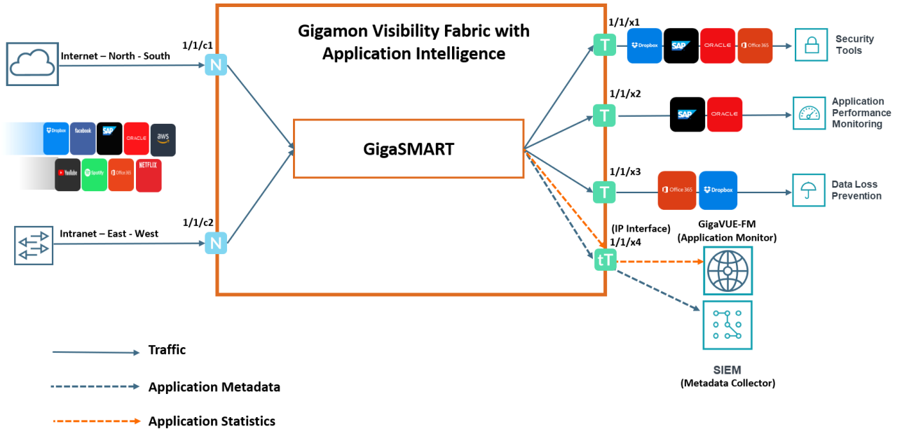
Figure 354: Application Intelligence Solution
