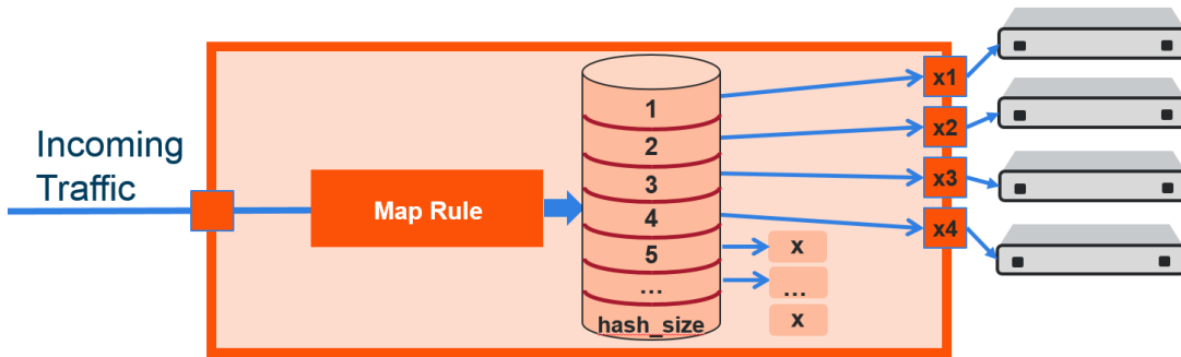
Figure 211: Controlled GigaStream Overview
