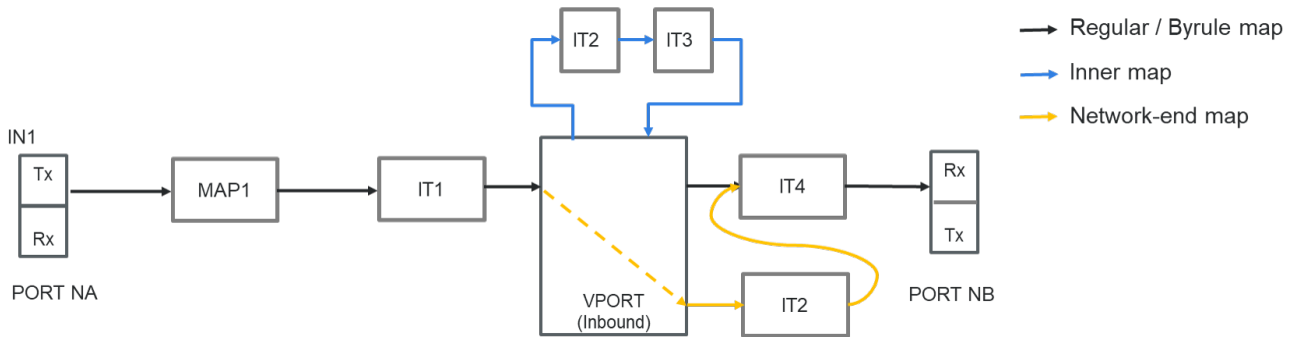
Figure 275: Flexible Inline Decryption Maps
