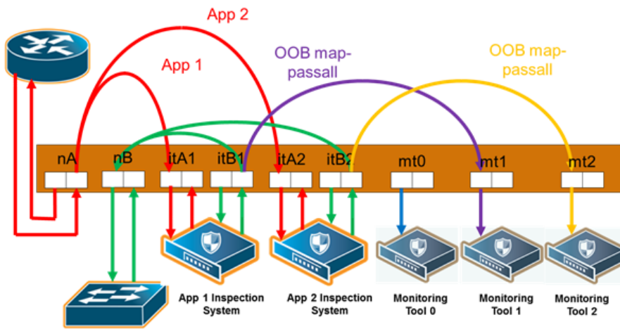
Figure 320: Out-of-Band Map Passalls
