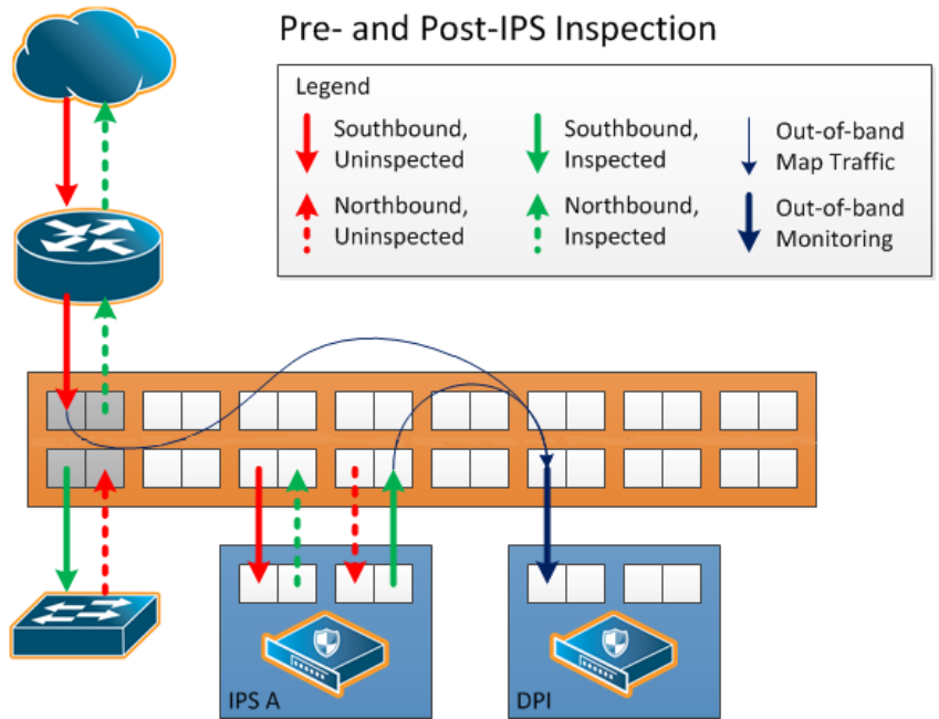
Figure 288: Out-of-Band Arrangement
